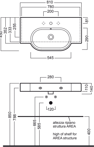
lavabo 81x45 washbasin 81x45
