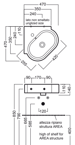
lavabo 47x47 destro washbasin 80x35 right
