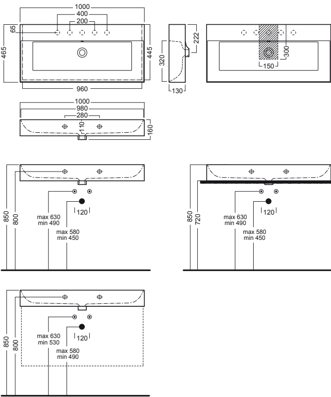
lavabo 100x46,5 washbasin 100x46,5
