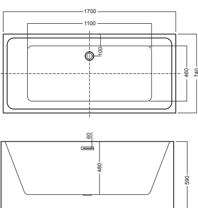
vasca 170x74 BT_02 bathtub 170x74 BT_02
