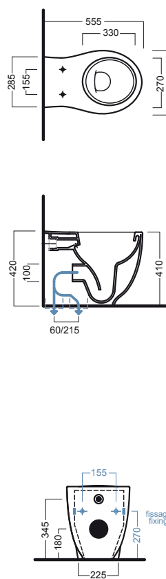
vaso filo muro_SCARICO TRASLATO back to wall wc_SHIFT DRAIN SYSTEM
