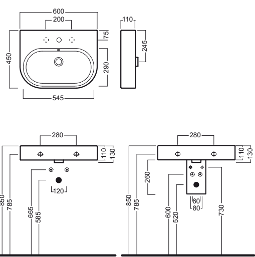
lavabo 60x45 washbasin 60x45
