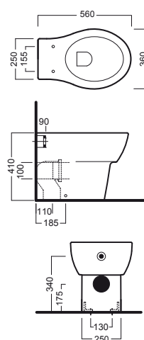
vaso filo muro back to wall wc
