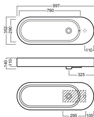
lavabo 100x35 washbasin 100x35
