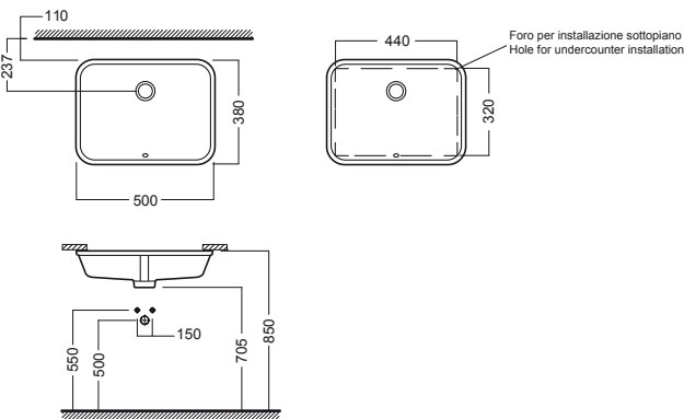
lavabo 50x38 washbasin 50x38
