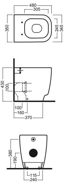
vaso filo muro back to wall wc
