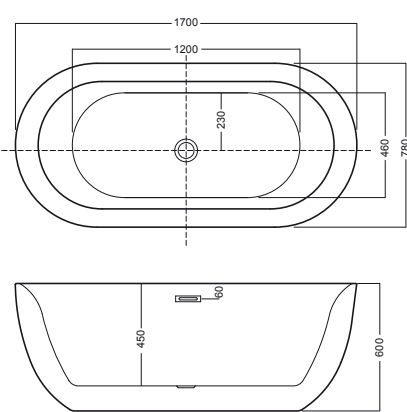
vasca 170x78 BT_01 bathtub 170x78 BT_01
