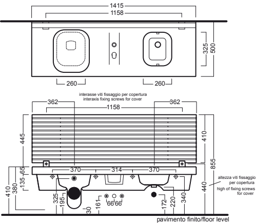
G-FULL 140 vaso a sinistra G-FULL 140 wc left
