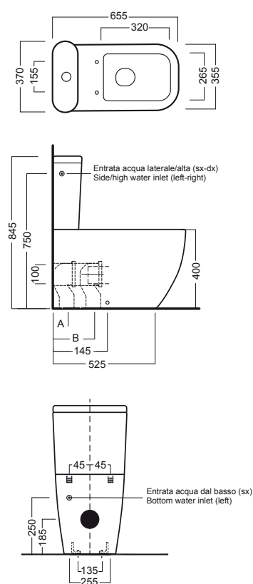
vaso monoblocco con cassetta coupled wc with cistern
