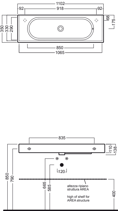
lavabo 110x35 washbasin 110x35
