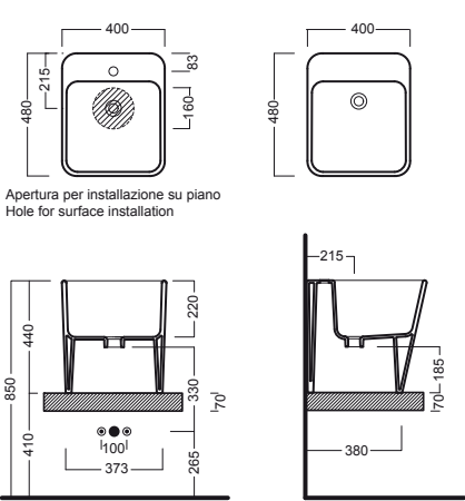
lavabo pilozzo in appoggio surface-mounted sink
