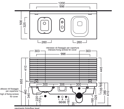
G-FULL 120 vaso a destra G-FULL 120 wc right
