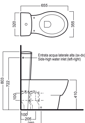
vaso monoblocco con cassetta coupled wc with cistern
