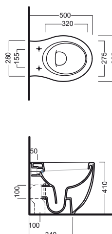
vaso filo muro_50 back to wall wc_50
