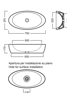
lavabo 75 da appoggio surface-mounted washbasin 75
