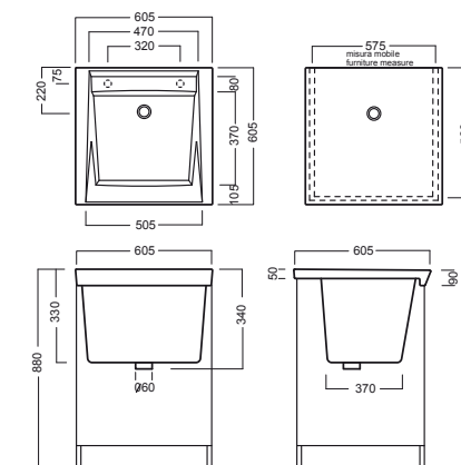
lavapanni SIXTY.LP SIXTY.LP laundry sink
